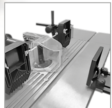
Working height adjustable from 0 to 40 mm Altura de trabajo regulable de 0 a 40 mm
